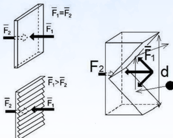
Fig.2 Ideas on redirecting of molecules
